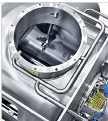
Cleaning nozzles for the WIP cleaning process
