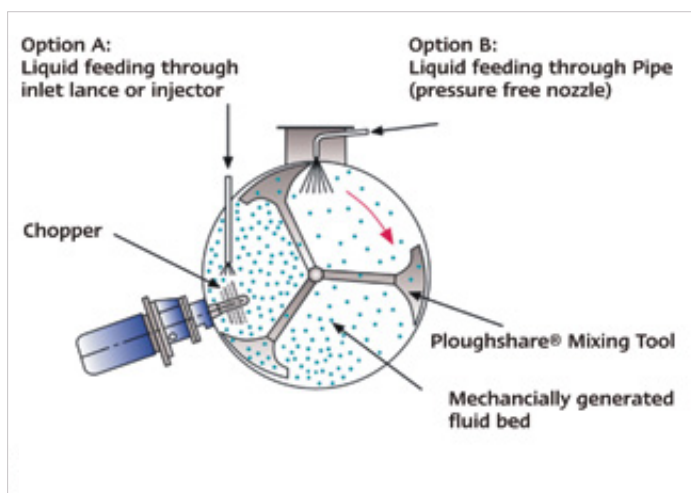
Some liquid addition possibilities in the Lödige Ploughshare® Mixer following the mixing and fluidisation process
