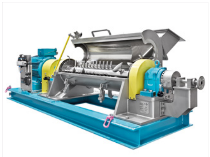
Ringlayer mixer CoriMix® Type CM 80
