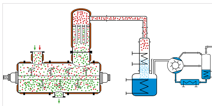
Principle of the vacuum shovel dryer DRUVATHERM®
