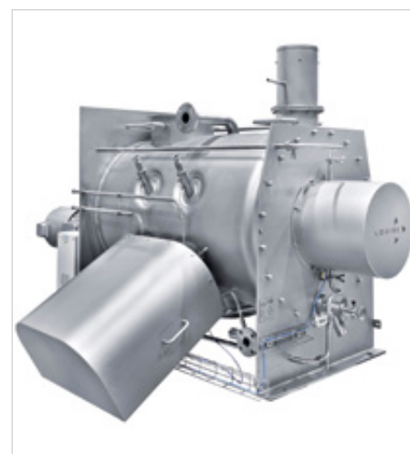
The cover hood above the bearing housing and motors creates an easy-to-clean surfaces
