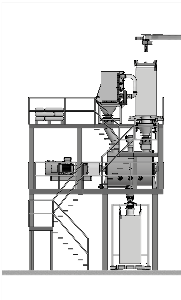
Mixing plant with manual infeed, big bag feeding and filling
